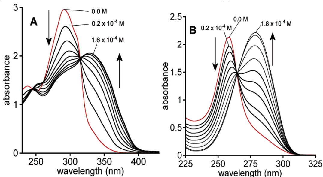
Figure 3. (A) Change of the UV–vis spectrum of 2 on titration with TFA. Conditions: [ 2 ] = 1.0 \times 10^{-4} M (unit concentration), [TFA] = 0.0 to 1.6 \times 10^{-4} M, CH 2 Cl 2 , 26 °C. Light path length 10 mm. (B) Change of the UV–vis spectrum of DMAP on titration with TFA. Conditions: [DMAP] = 1.0 \times 10^{-4} M, [TFA] = 0 to 1.8 \times 10^{-4} M, CH 2 Cl 2 , 26 °C. Light path length 10 mm. Red-colored lines represent the spectra in the absence of TFA.
