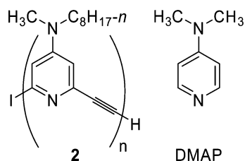
Figure 2. Structures of basic poly( m -ethynylpyridine) 2 and DMAP.
